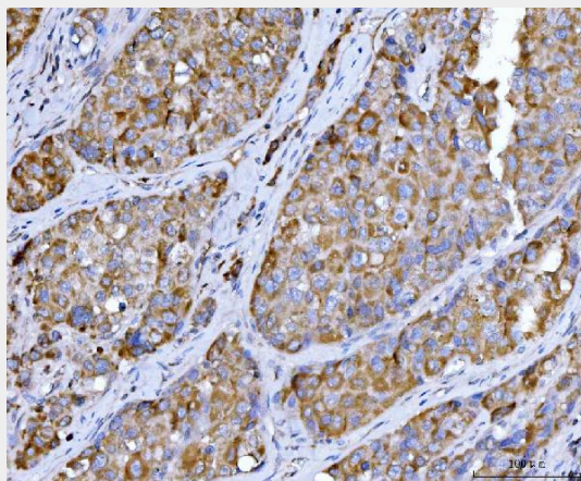
Figure 3. IHC analysis of Beclin 1 using anti-Beclin 1 antibody (M00327-2). Beclin 1 was detected in a paraffin-embedded section of human hepatocellular carcinoma tissue. Heat mediated antigen retrieval was performed in EDTA buffer (pH 8.0, epitope retrieval solution). The tissue section was blocked with 10% goat serum. The tissue section was then incubated with 2 µg/ml mouse anti-Beclin 1 Antibody (M00327-2) overnight at 4°C. Peroxidase Conjugated Goat Anti-mouse IgG was used as secondary antibody and incubated for 30 minutes at 37°C. The tissue section was developed using HRP Conjugated Mouse IgG Super Vision Assay Kit (Catalog # SV0001) with DAB as the chromogen.
